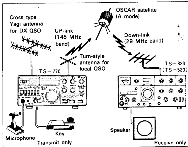
Fig. 16 Example of OSCAR Operation
