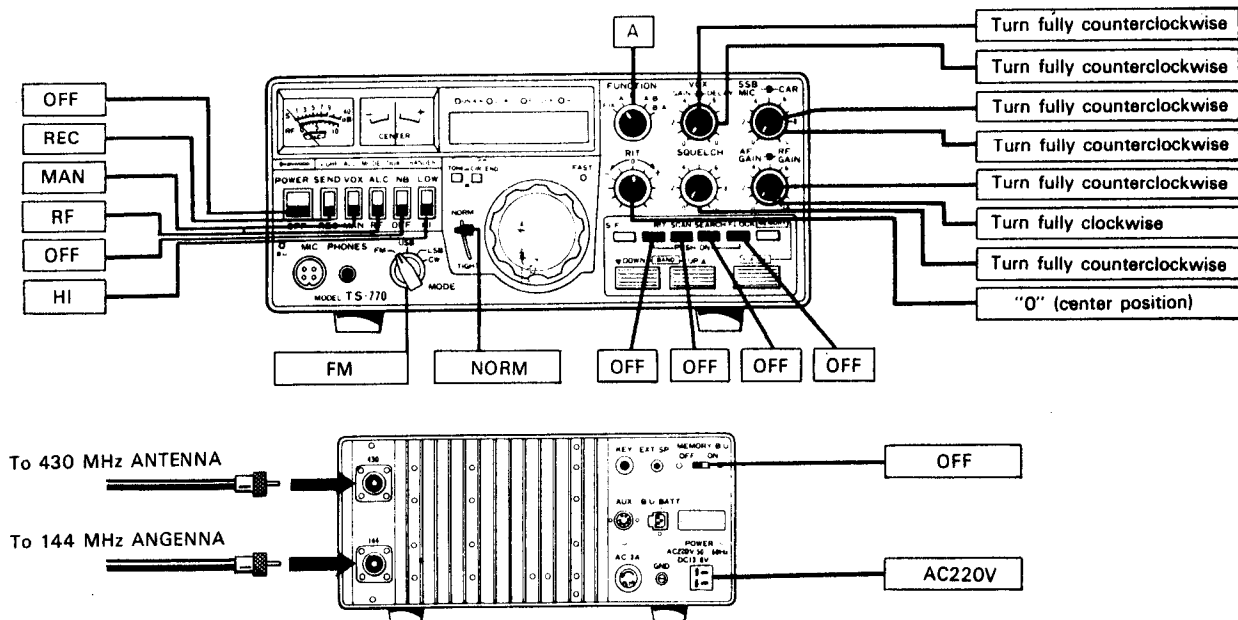
Fig. 9 Pre-setting for Reception
